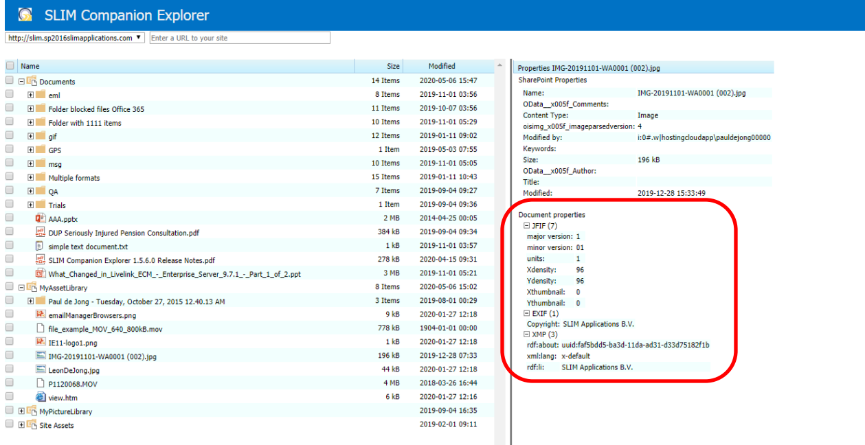
Figure 13. List with properties available in the selected file.
